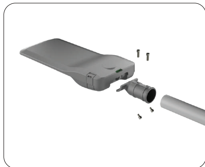
Horizontal installation
